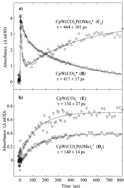
Figure 2. Kinetic plots for (a) \text{CpW}(\text{CO})_3\text{P}(\text{OMe})_3^\bullet and \text{CpW}(\text{CO})_3^\bullet , and (b) \text{CpW}(\text{CO})_3^- and \text{CpW}(\text{CO})_3\text{P}(\text{OMe})_3^+ following 400 nm photolysis of [\text{CpW}(\text{CO})_3]_2 in a 1.6 M solution of \text{P}(\text{OMe})_3 with \text{CH}_2\text{Cl}_2 . Lines represent fits to the data (see text).
