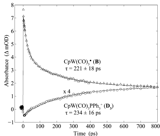
Figure 7. Kinetic plots for \text{CpW}(\text{CO})_3^{\bullet} and \text{CpW}(\text{CO})_3\text{PPh}_3^+ following 400 nm photolysis of [\text{CpW}(\text{CO})_3]_2 in a 1.3 M solution of \text{PPh}_3 in \text{CH}_2\text{Cl}_2 . 39 Lines represent fits to the data (see text).
