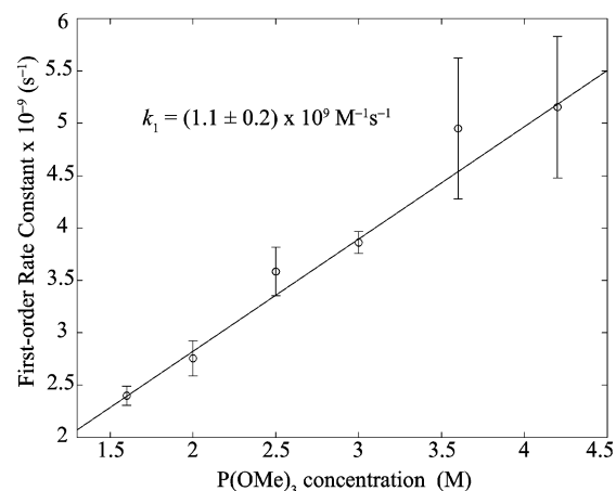
Figure 3. Dependence of the pseudo first-order rate constant for 19e intermediate formation on the concentration of Lewis base P(OMe) 3 .
