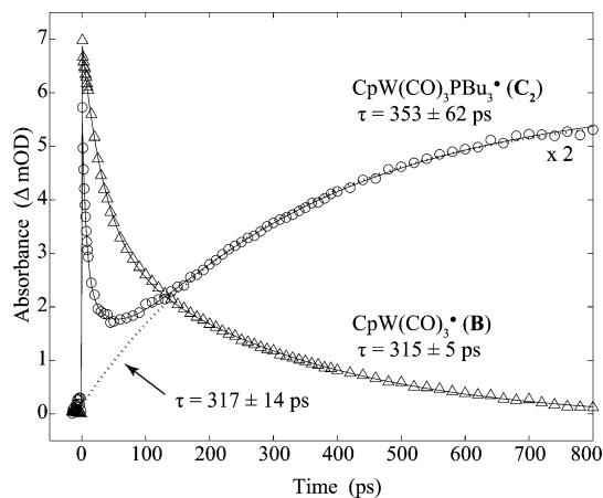
Figure 5. Kinetic plots for \text{CpW}(\text{CO})_3\text{PBU}_3^* and \text{CpW}(\text{CO})_3^* following 400 nm photolysis of [\text{CpW}(\text{CO})_3]_2 in a 2.0 M solution of \text{PBU}_3 in \text{CH}_2\text{Cl}_2 . Absorbance values for \text{CpW}(\text{CO})_3\text{PBU}_3^* are scaled by a factor of 2 for clarity. Lines represent fits to the data (see text).
